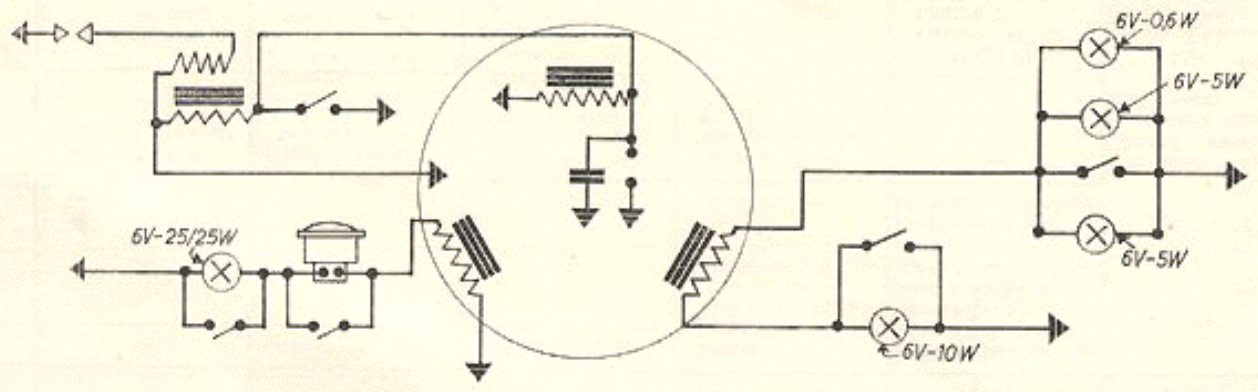
FIG. 38B. WIRING DIAGRAM, 180 SS WITHOUT BATTERY
