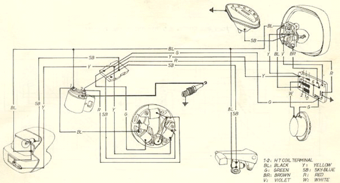
FIG. 38A. Wiring Diagram, VSB 1 WITHOUT BATTERY
