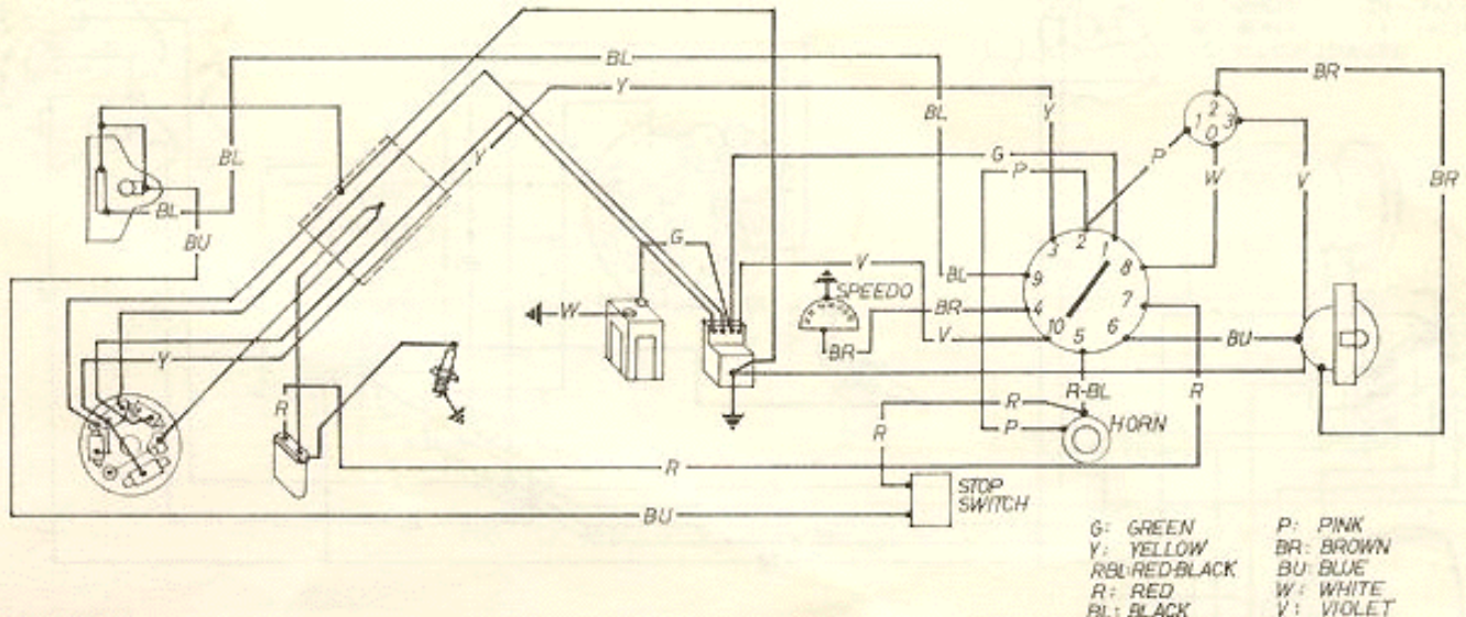
FIG. 37b. WIRING DIAGRAM, G.S. MODELS VSB 1 SERIES 2
